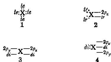
Fig. 1. Octet structures and orbital hybridization.
