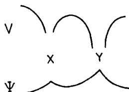
FIG. 6. One-dimensional model of a polar bond.
