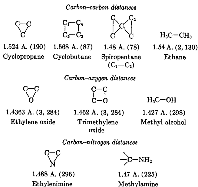
FIG. 8. Interatomic distances in several small-ring compounds (113).
